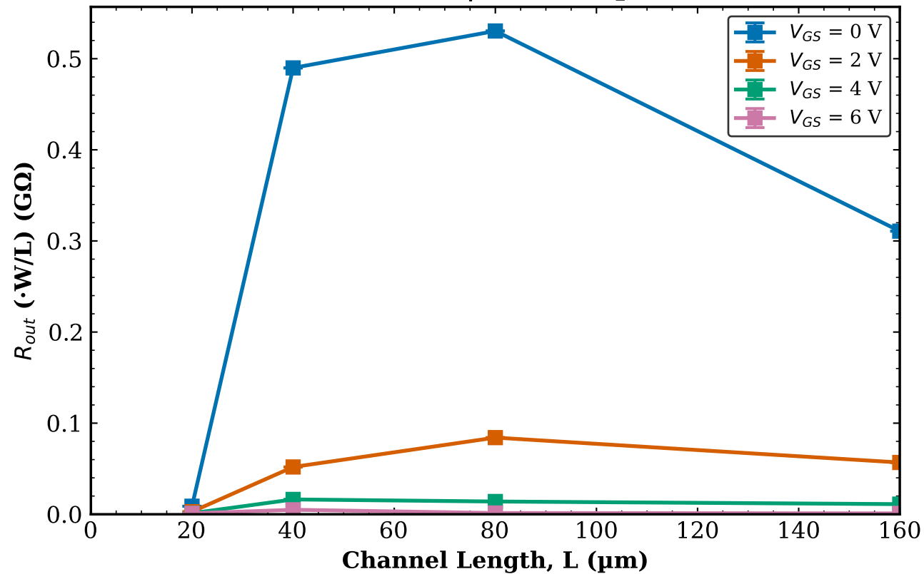
TFT2 Transistor 1 R_{out} vs L | W = 50\text{ }\mu\text{m}
